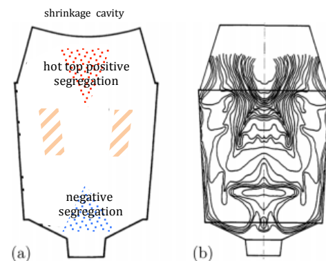
FIGURE 3A SCHEMATIC OF 180 TONNE STEEL INGOT[20]
