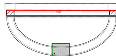
FIGURE 5 LOCATION OF SAMPLE SECTIONS FOR TC SURPLUS TEST RING ■ MID-SHELL LOCATIONS ■
