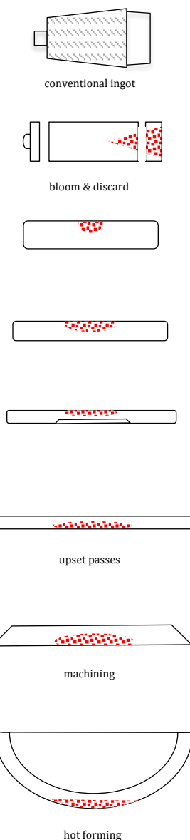
FIGURE 3B FORGING PROCESS
